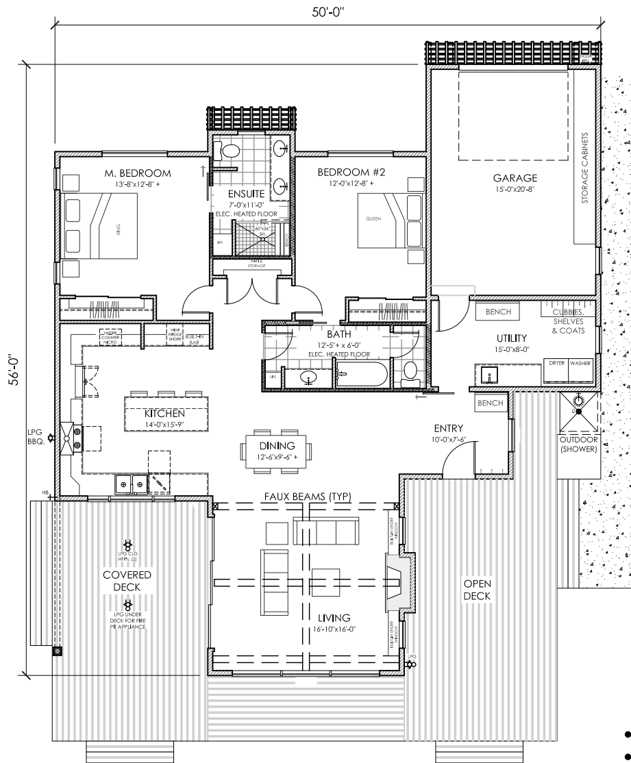
MAIN FLOOR PLAN
