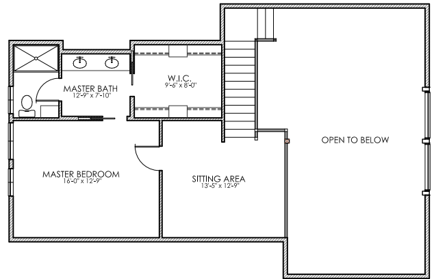
TOP FLOOR PLAN
