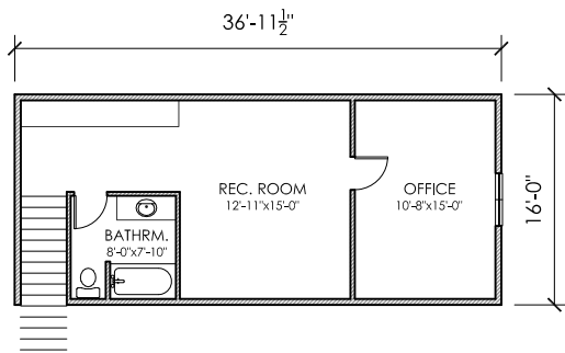
TOP FLOOR PLAN
