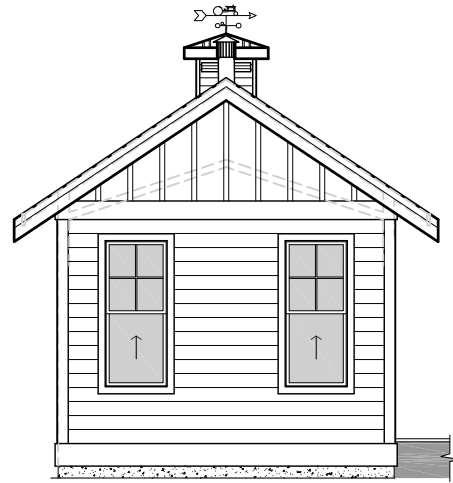
SIDE ELEVATIONS
