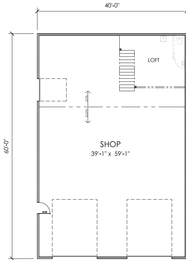
FLOOR PLAN
