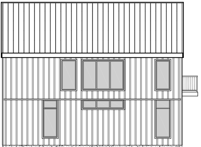
ELEVATIONS
