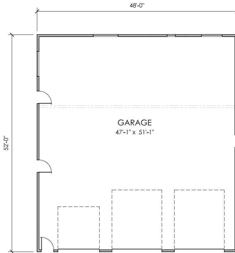
FLOOR PLAN
