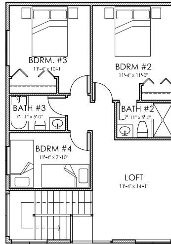
TOP FLOOR PLAN
