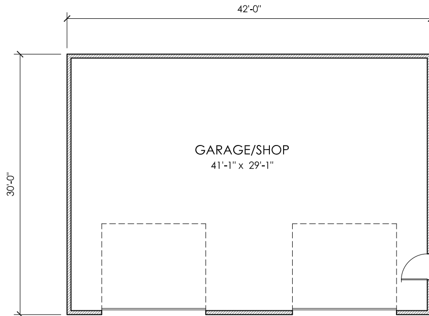
FLOOR PLAN
