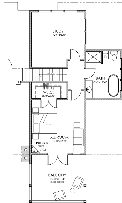
TOP FLOOR PLAN
