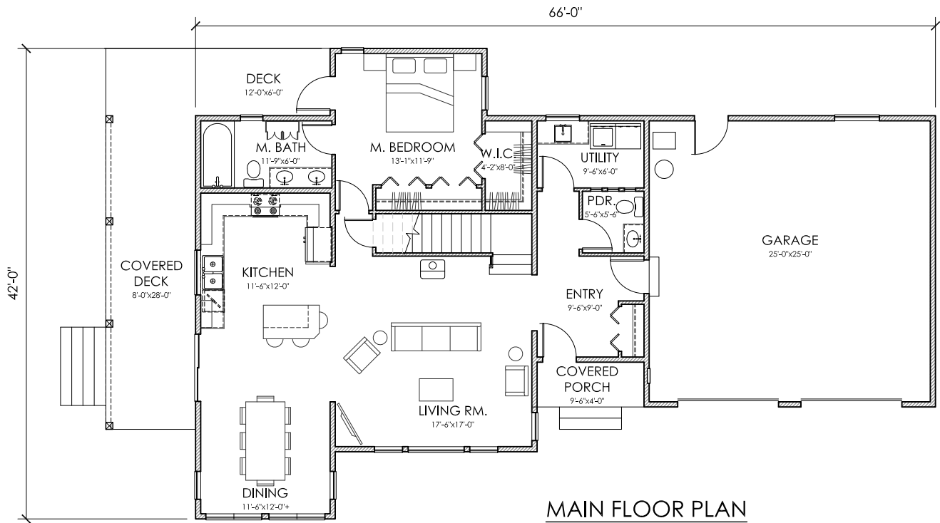
TOP FLOOR PLAN
