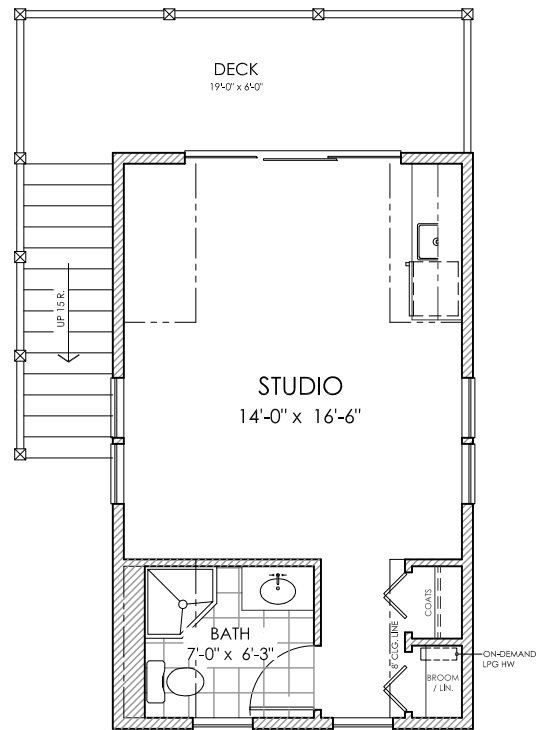
TOP FLOOR PLAN
