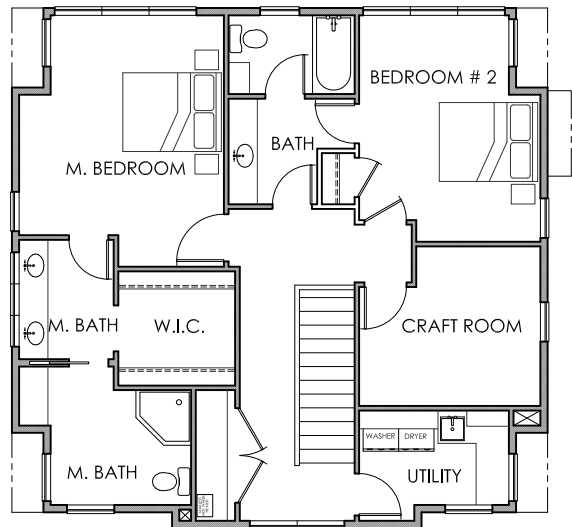
TOP FLOOR PLAN
