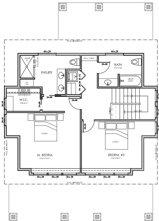
TOP FLOOR PLAN
