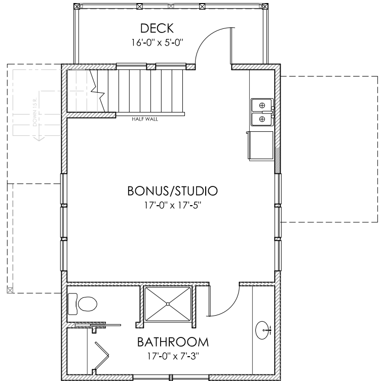
TOP FLOOR PLAN
