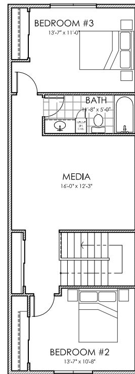
TOP FLOOR PLAN
