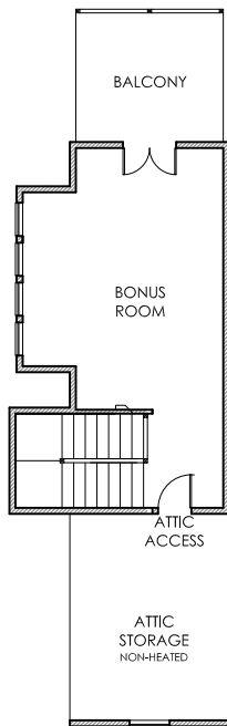
TOP FLOOR PLAN
