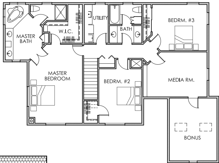
TOP FLOOR PLAN
