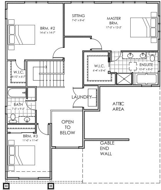
TOP FLOOR PLAN
