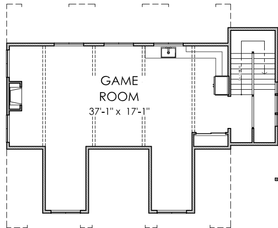
TOP FLOOR PLAN
