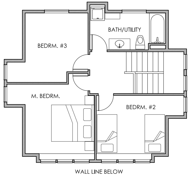
TOP FLOOR PLAN
