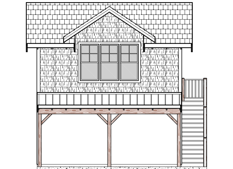
ELEVATIONS
