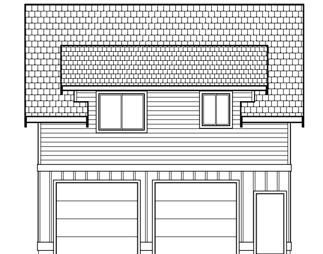
ELEVATIONS
