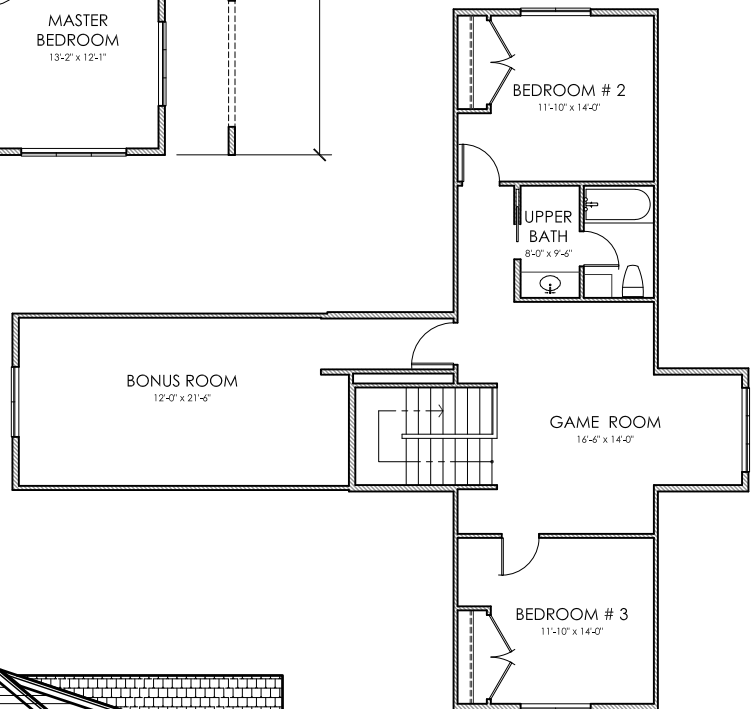
TOP FLOOR PLAN
