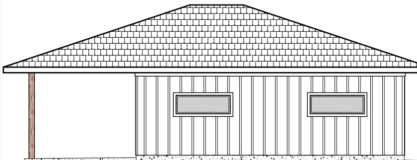
SIDE ELEVATION
