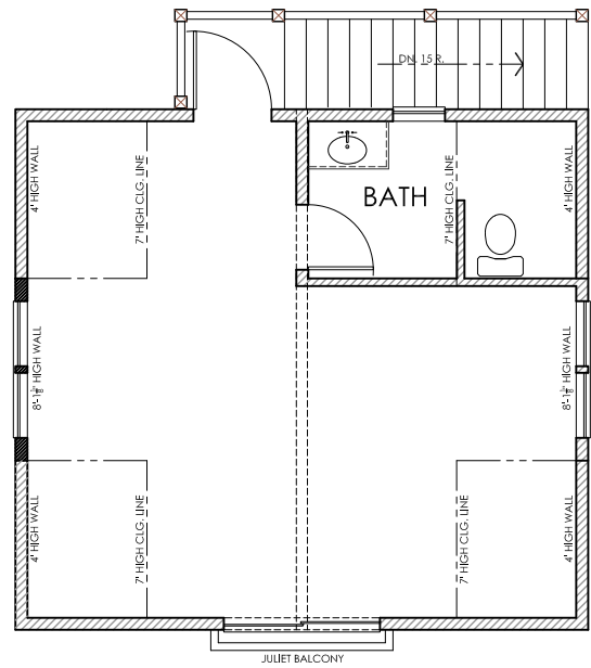
TOP FLOOR PLAN
