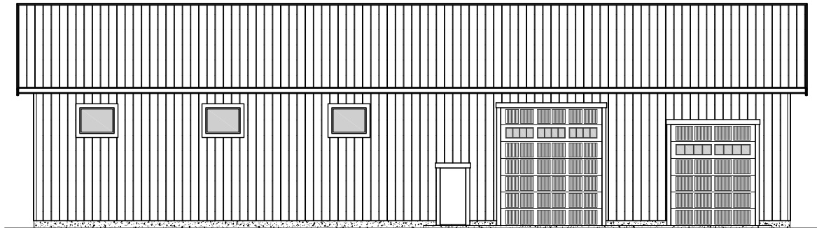
FRONT ELEVATION
