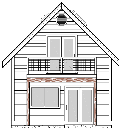
REAR ELEVATION
