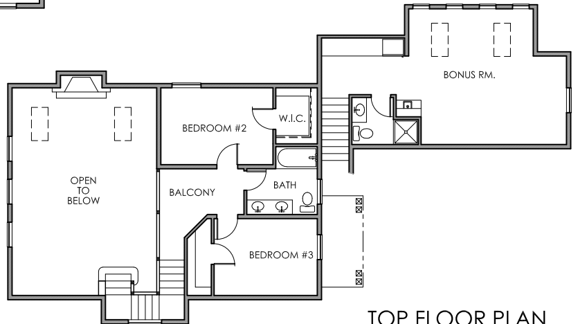
TOP FLOOR PLAN
