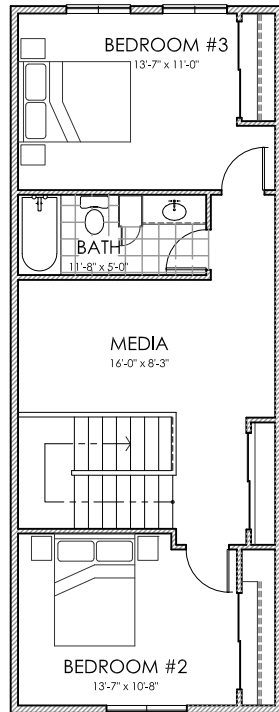
TOP FLOOR PLAN
