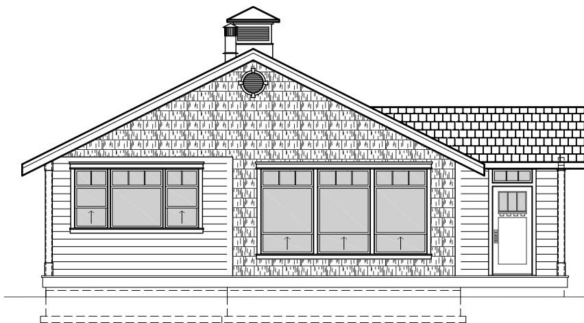
FRONT ELEVATION
