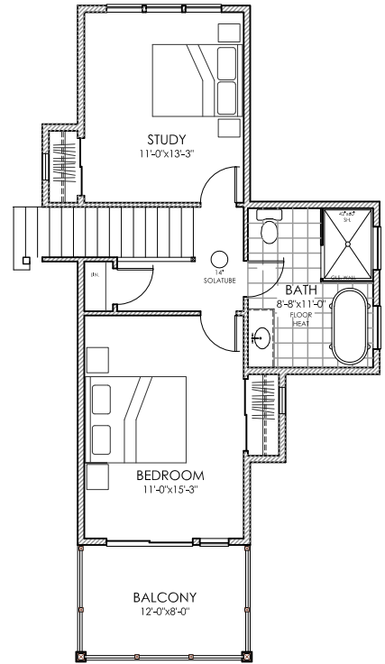
TOP FLOOR PLAN
