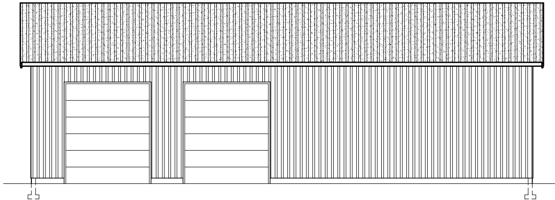
FRONT ELEVATION
