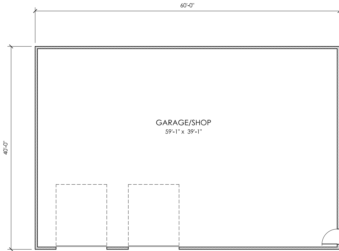
FLOOR PLAN
